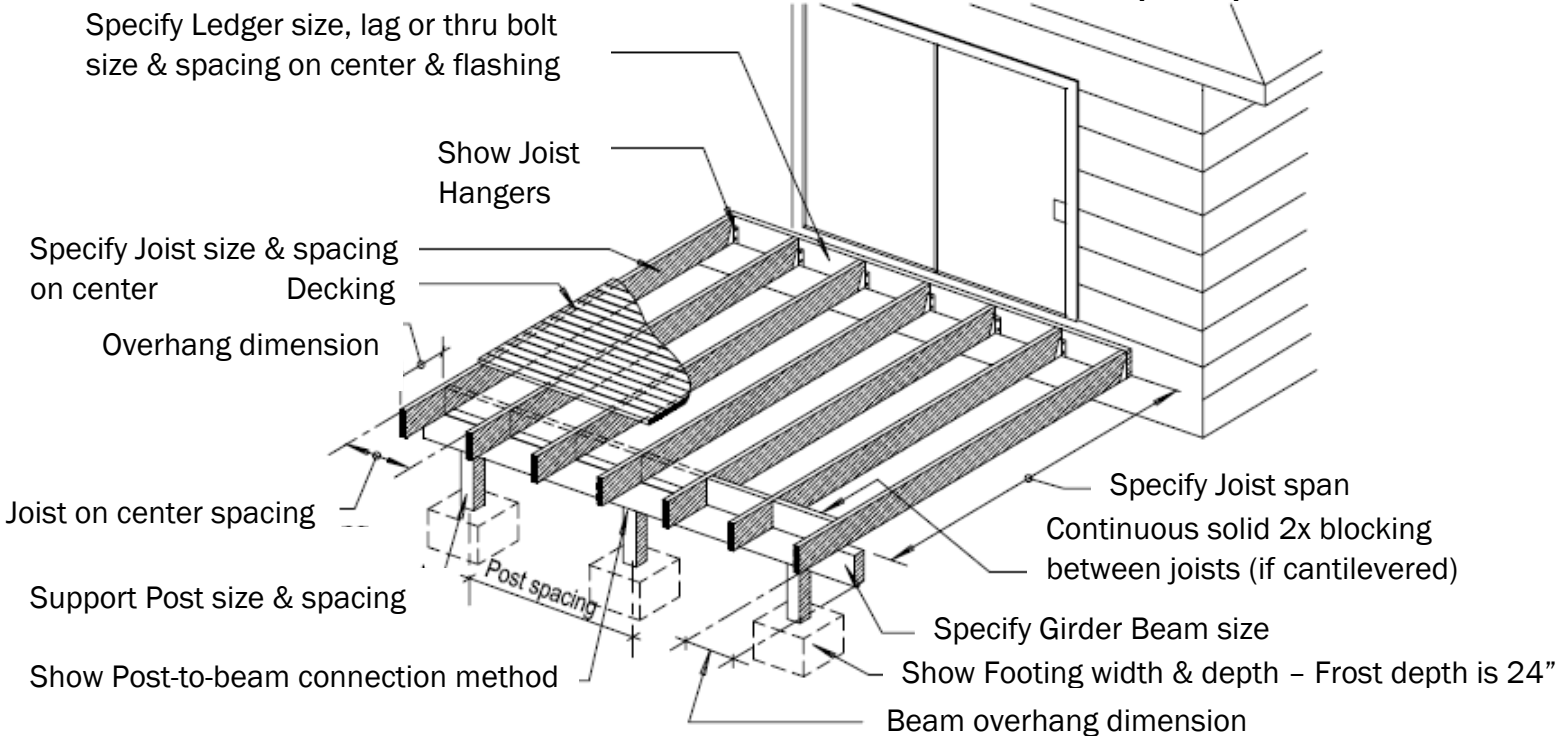
Typical Deck
